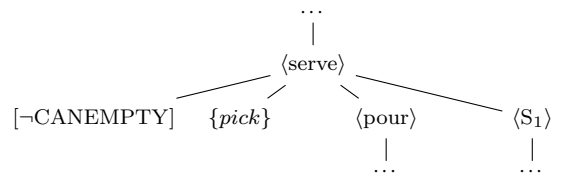
Fig. 3: The first production from the grammar in figure 1 represented as part of a parse tree
